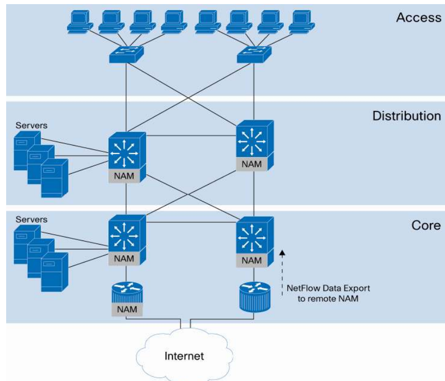
Figure 4. Deploying Cisco NAMs for Voice Monitoring in the Campus Network
