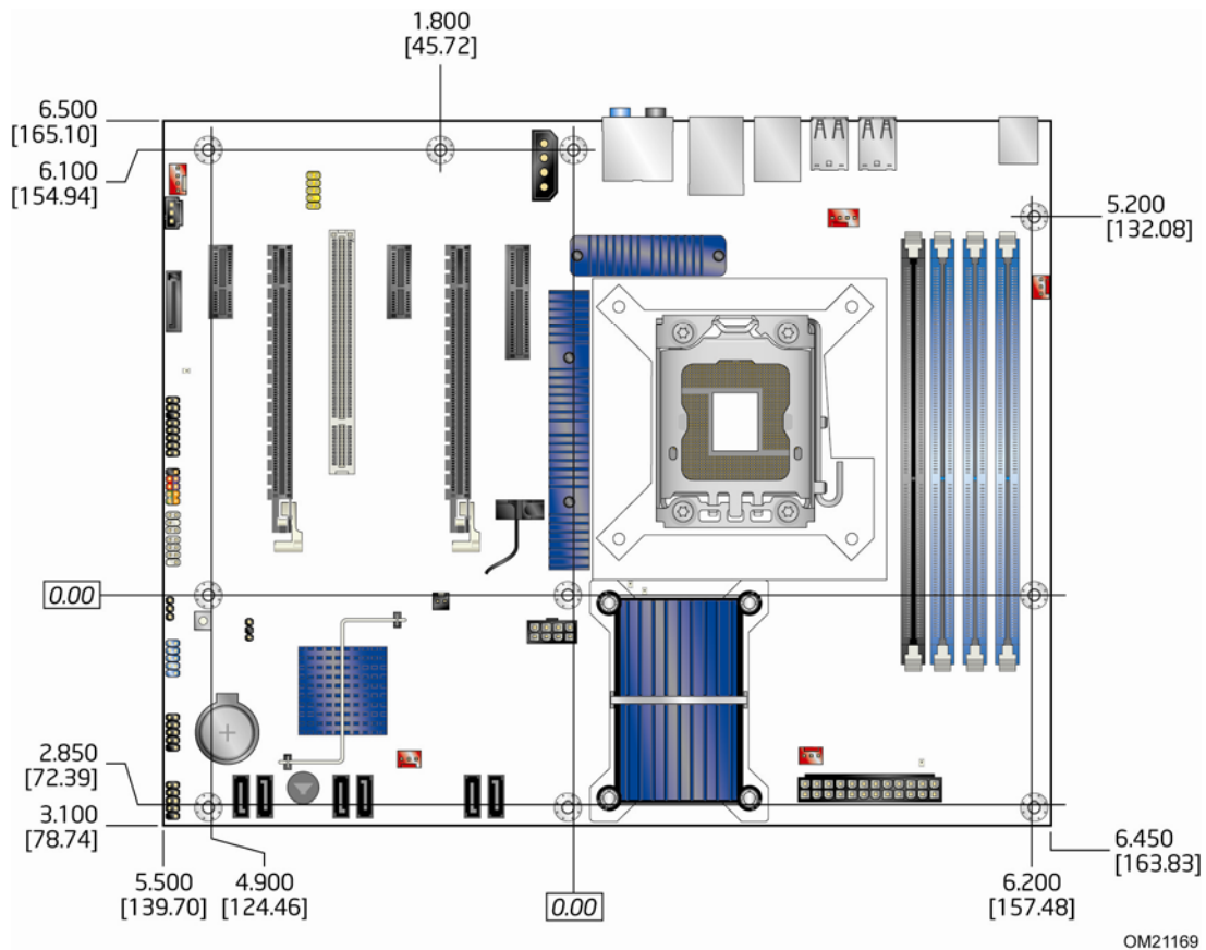
Figure 16. Board Dimensions
