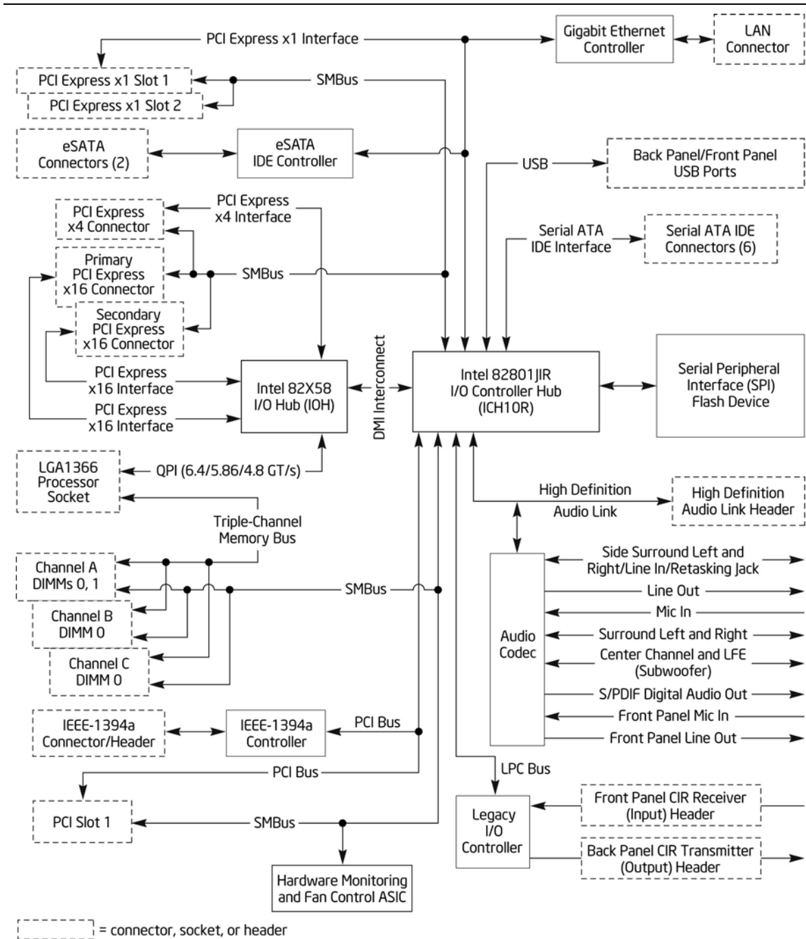
Figure 2. Block Diagram
