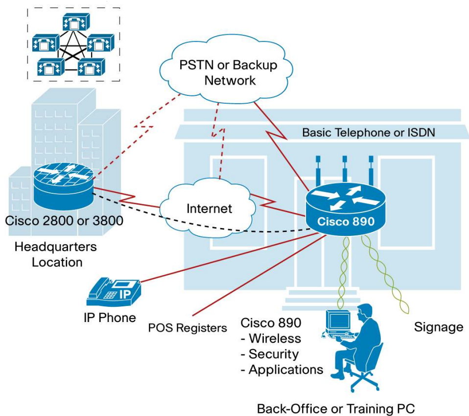
Figure 5. High Availability
