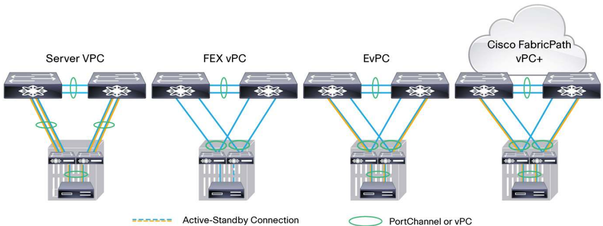
Figure 5. Cisco Nexus B22 Design Scenarios, from Left to Right: Server vPC, Fabric Extender vPC, Enhanced vPC, and vPC+
