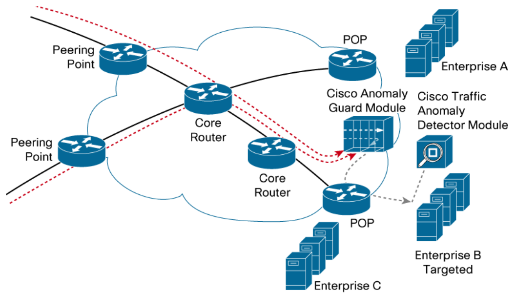
Figure 5. Cisco DDoS Anomaly Detection and Mitigation in a Centralized Provider Scrubbing Center
