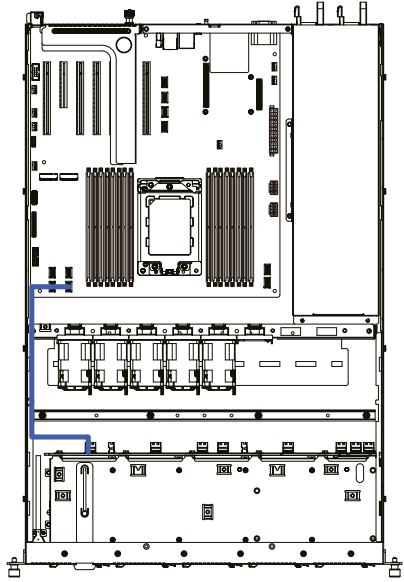
U.2 NVMe to HDD Back Plane Board Cable (NVMe1)
