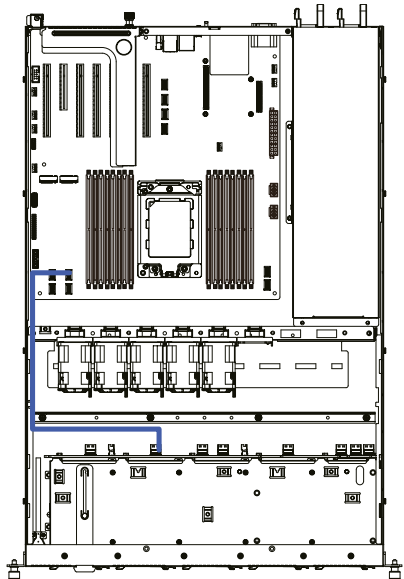
U.2 NVMe to HDD Back Plane Board Cable (NVMe3)
